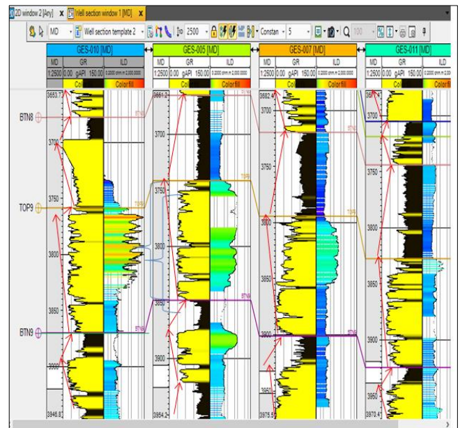
Fig 5: Correlation of sandstone units across the four wells from the log trends.
